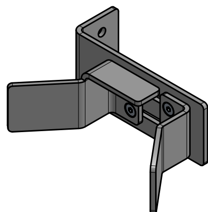
Large Gate Catch 1:4
